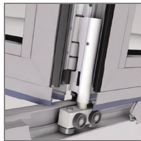
Bottom Roller & Track
